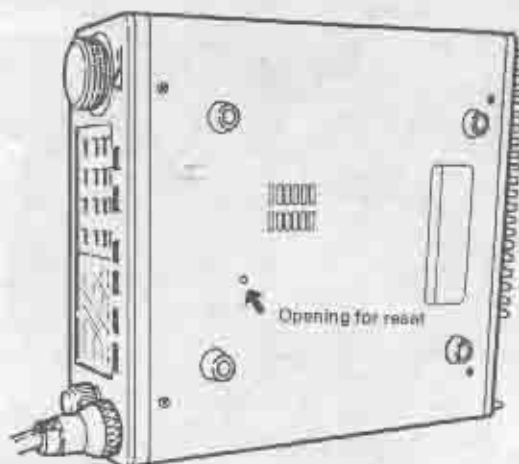
Fig 1-4 Microprocessor reset
